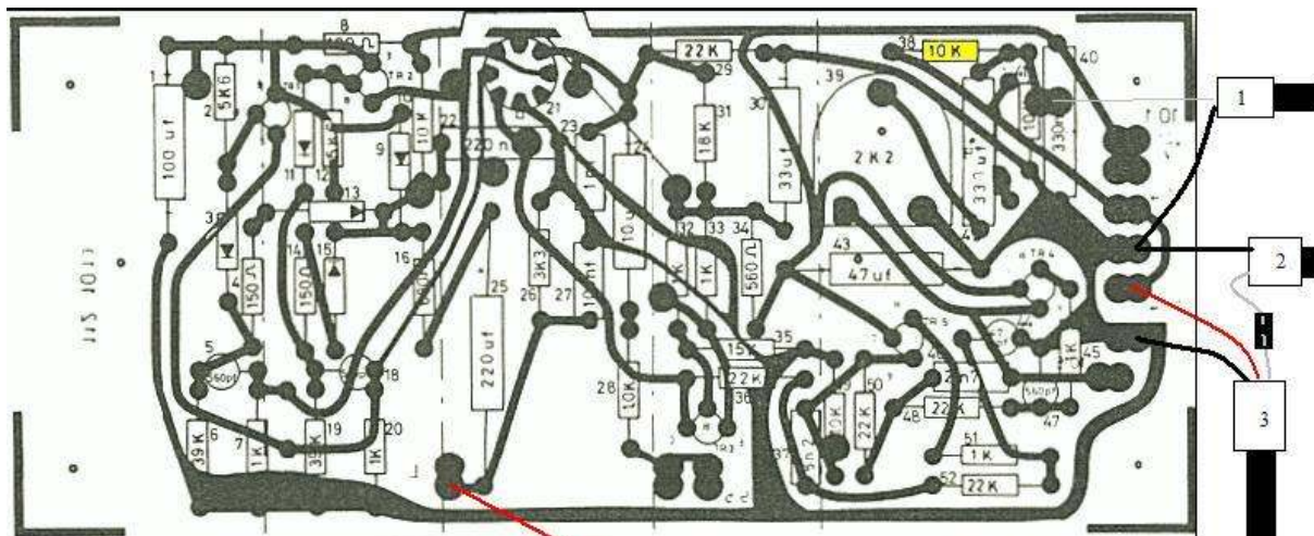
MODULATOR BOARD
