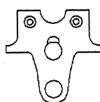
Festiniog wooden slate wagon Axlebox
