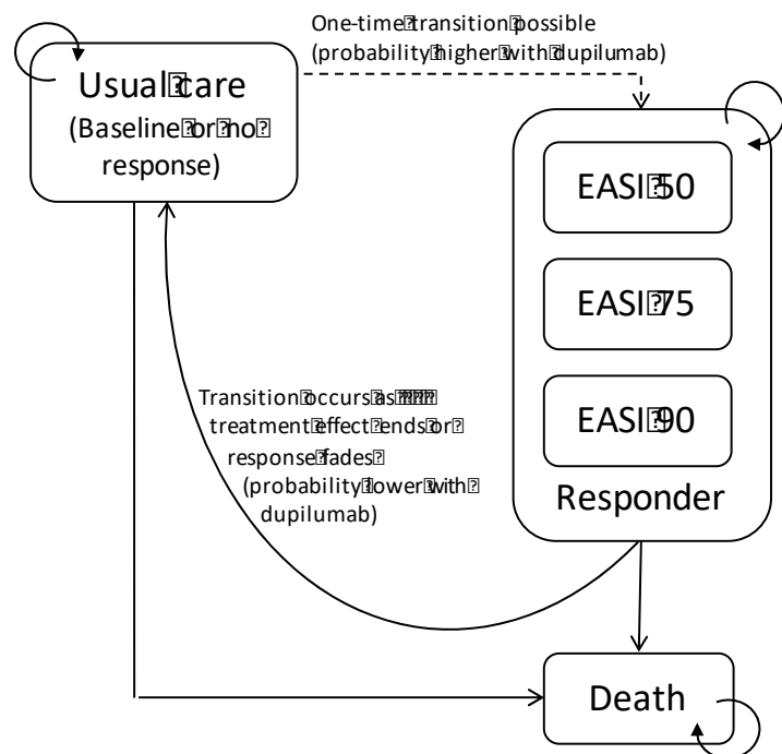
Figure 3. Markov Model Structure
