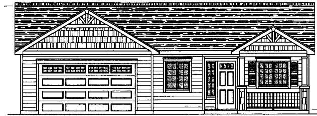
Front Elevation A1
